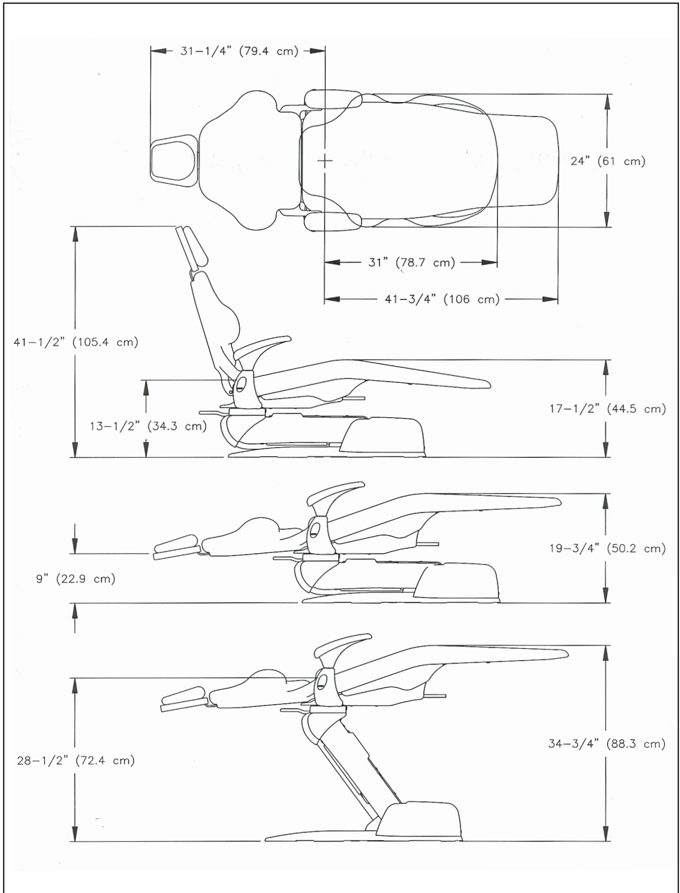
ALLIANT PATIENT CHAIR DIMENSIONS
